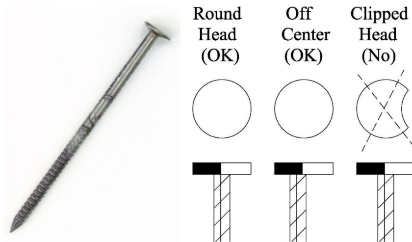
Figure 2. Use 8d ring-shank nails when attaching roof sheathing. Research indicates that panels attached with ring-shank nails have about twice the uplift capacity compared to panels attached with the same size smooth-shank nails.
